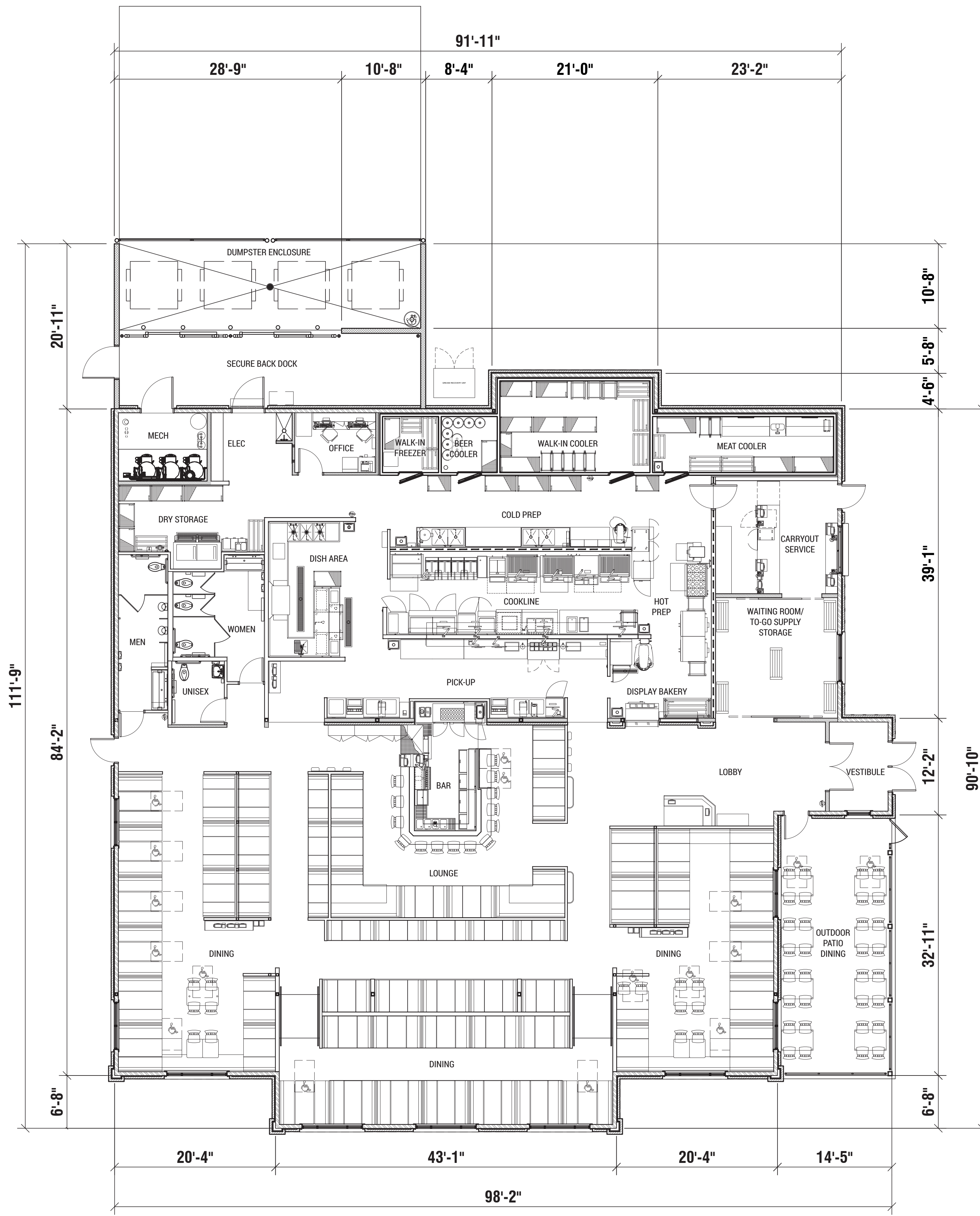
FLOOR PLAN
